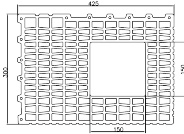
Figure 7 – Brique Poteau
