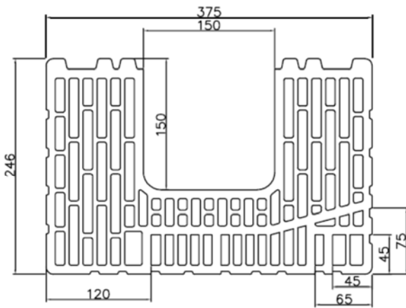
Poteau R37
