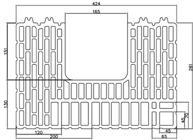
Poteau R42
