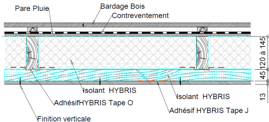
Annexe 5. Figure : 2. COUPE H-H principe 2/3 – 1/3
